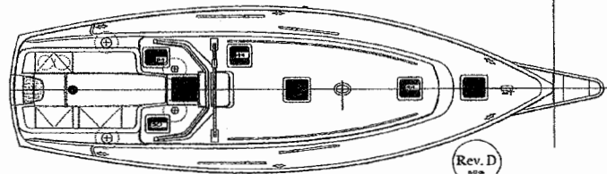
PRELIMINARY concept drawing for Pacific Seacraft 38' Cruising Yacht
